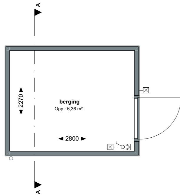
00 Begane grond
