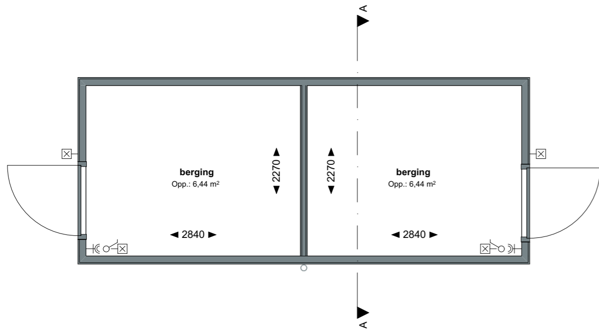
00 Begane grond
