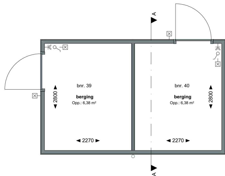
00 Begane grond
