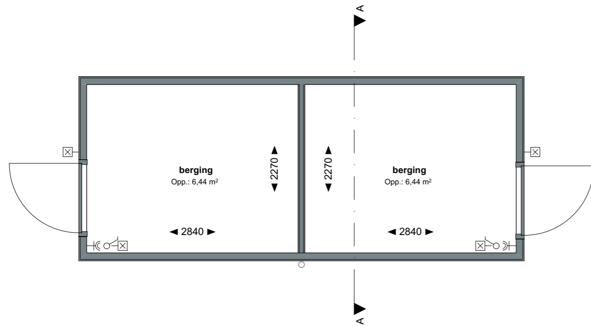
00 Begane grond
