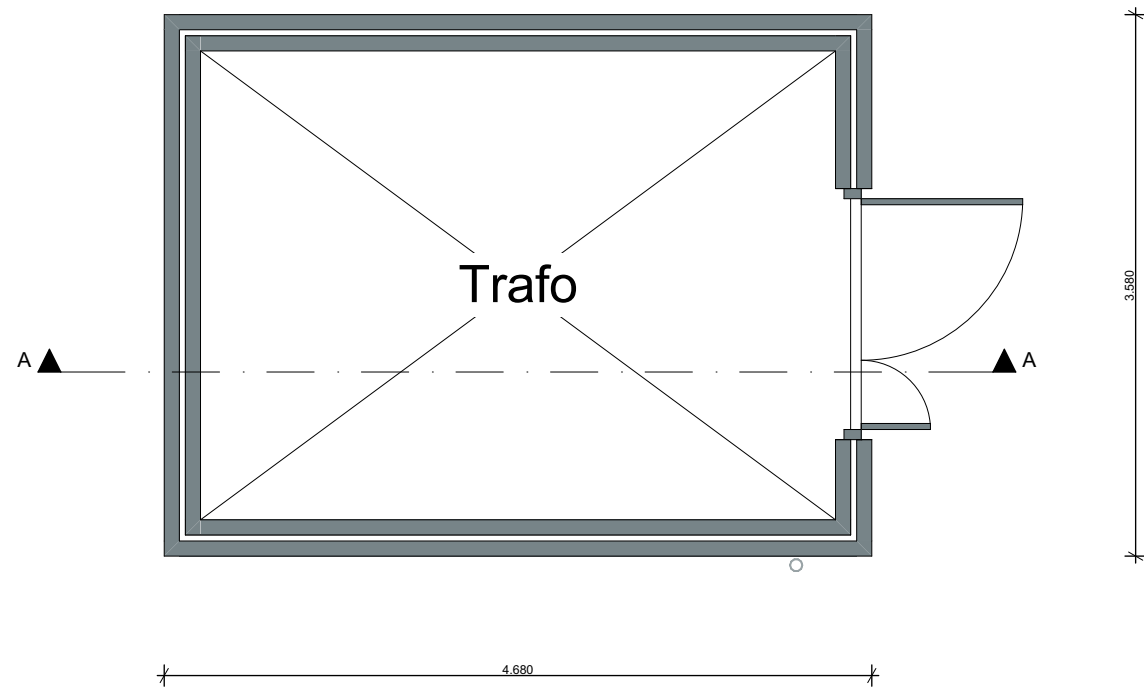
00 Begane grond
